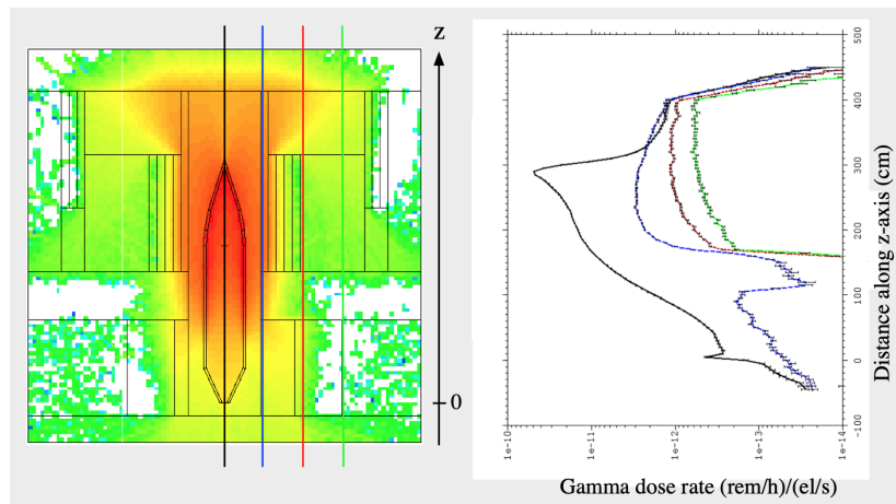
FIGURE 11. Dose rate along the z-direction in the plane through the collector central axis and at different distances from the axis.
