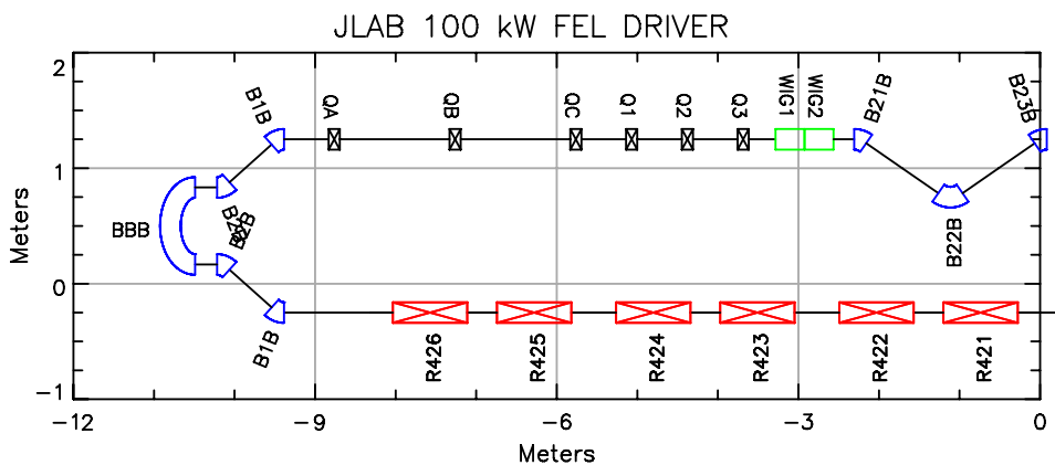
Figure 10.4: Example Floor Plan drawing.
