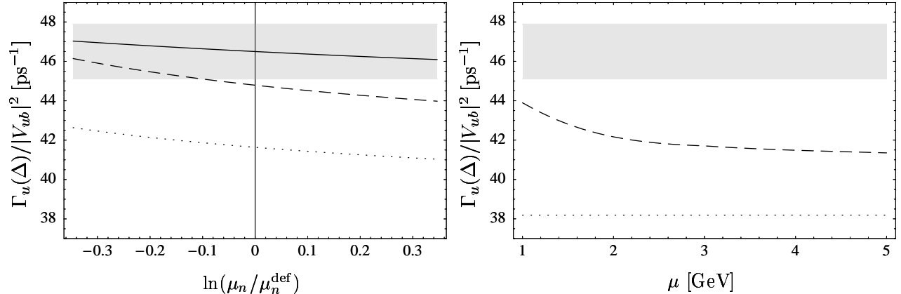
Figure 2: Convergence of the perturbative series and residual scale dependence. LEFT : RG-improved results at LO (dotted), NLO (dashed), and NNLO (solid) as a function of the scales \mu_i , \mu_h , \bar{\mu} , which are varied simultaneously about their default values. RIGHT : Fixed-order results at tree-level (dotted) and one-loop order (dashed).
