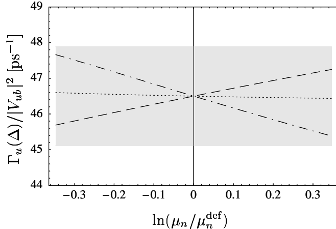
Figure 1: Residual scale dependence of \Gamma_u(\Delta) for \Delta = 0.65 GeV. The dashed line depicts the variation of \mu_h about its default value m_b/\sqrt{2} , the dash-dotted line the variation of \mu_i about 1.5 GeV, and the dotted line the variation of \bar{\mu} also about 1.5 GeV. The highlighted area shows the combined perturbative uncertainty.
