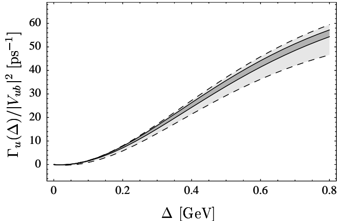
Figure 3: Perturbative uncertainties on \Gamma_u(\Delta) encountered when using the weight function W(\Delta, P_+) (dark gray) or \widetilde{W}(\Delta, P_+) (light gray). In the latter case, the normalization of the photon spectrum is chosen such that the two predictions agree at \Delta = 0.65 GeV for central values of the matching scales.
