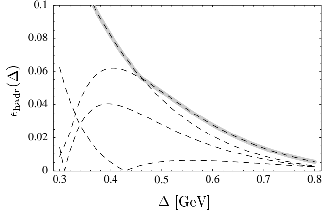
Figure 4: Estimates for the hadronic uncertainty \epsilon_{\text{hadr}}(\Delta) obtained from a scan over models for the subleading shape functions. The dashed lines correspond to the individual results for the four h_i(\hat{\omega}) functions suggested in [7]. The thick solid line, which covers one of the dashed lines, shows the maximum effect.
