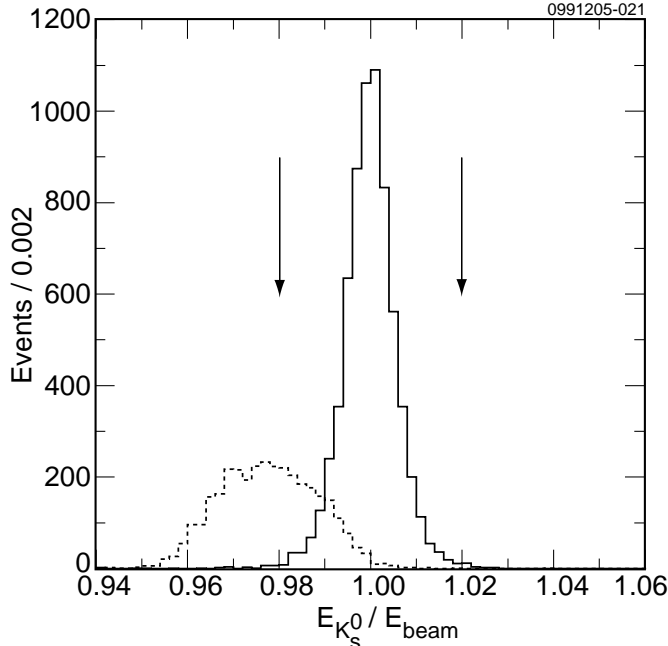
FIG. 1: The scaled K_S^0 energy ( E_{K_S^0}/E_{\text{beam}} ) distribution for the \psi(3770) simulation samples corresponding to the signal (solid histogram) and radiative return (dotted histogram) processes using arbitrary normalization. The arrows mark the signal region.
