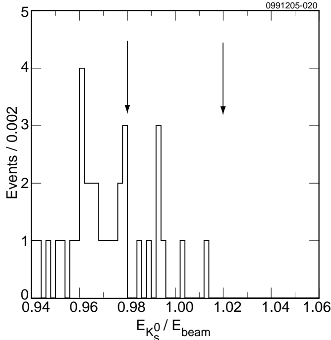
FIG. 2: The scaled K_S^0 energy ( E_{K_S^0}/E_{\text{beam}} ) distribution for the \psi(3770) \rightarrow K_S^0 K_L^0 decay in 281 \text{ pb}^{-1} of data. The arrows mark the signal region.
