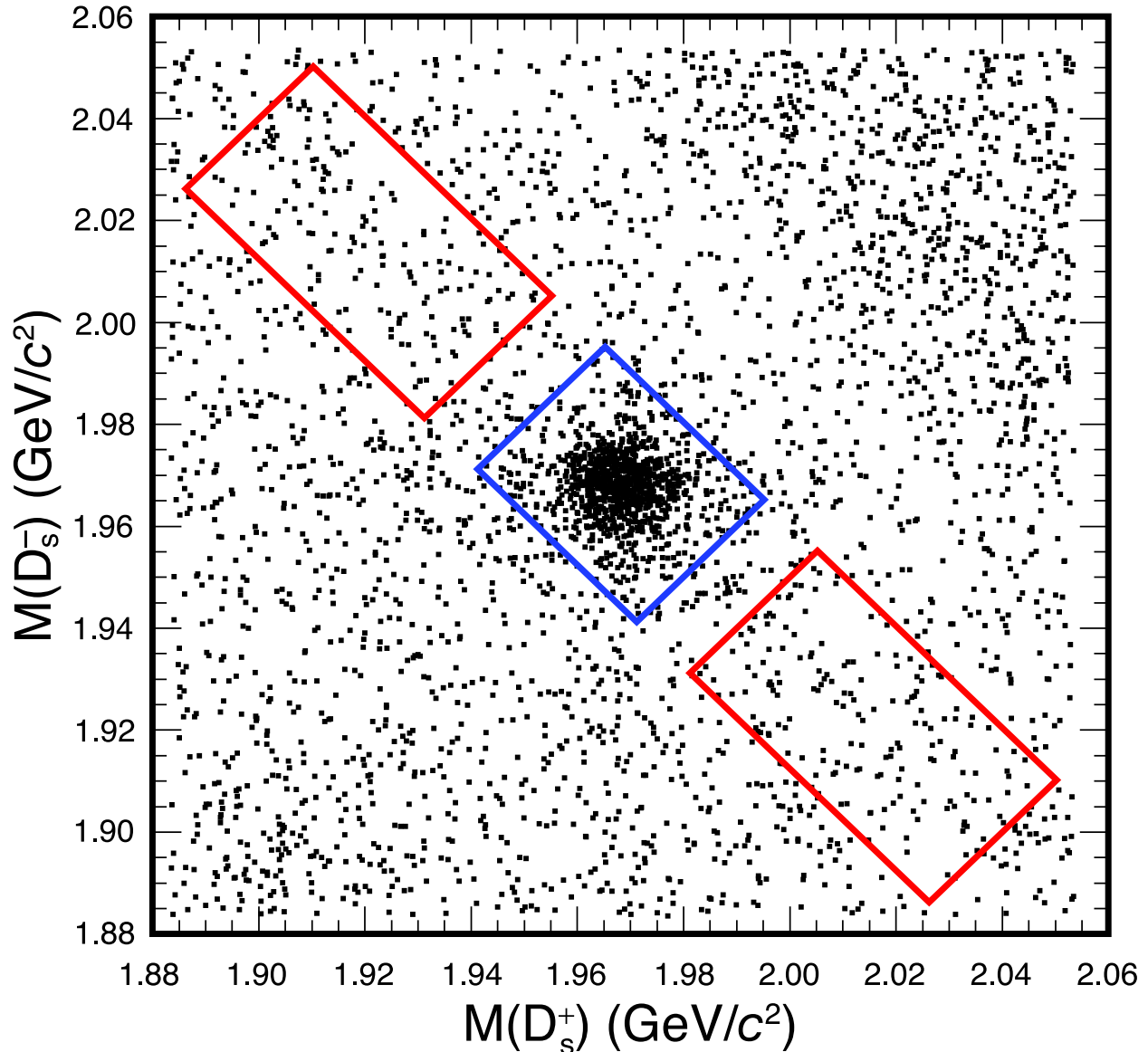
FIG. 2: (Color online) Masses of the D_s^- and D_s^+ candidates for all 64 DT modes in data. The rectangles show the signal region (center) and two sideband regions (diagonally offset). There are 1089 events in the signal region and 339 events in the combined sideband regions.
