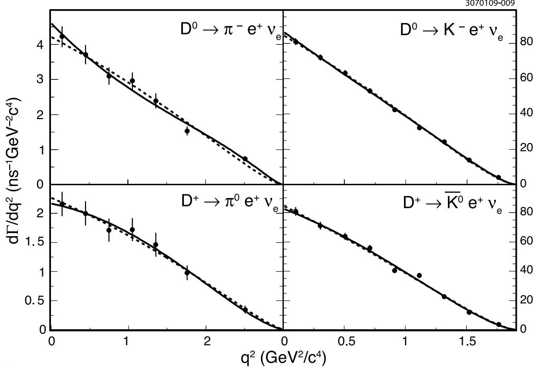
FIG. 9: Individual form factor fits to data (points) using 2-parameter (dashed) and 3-parameter (solid) series expansions.
