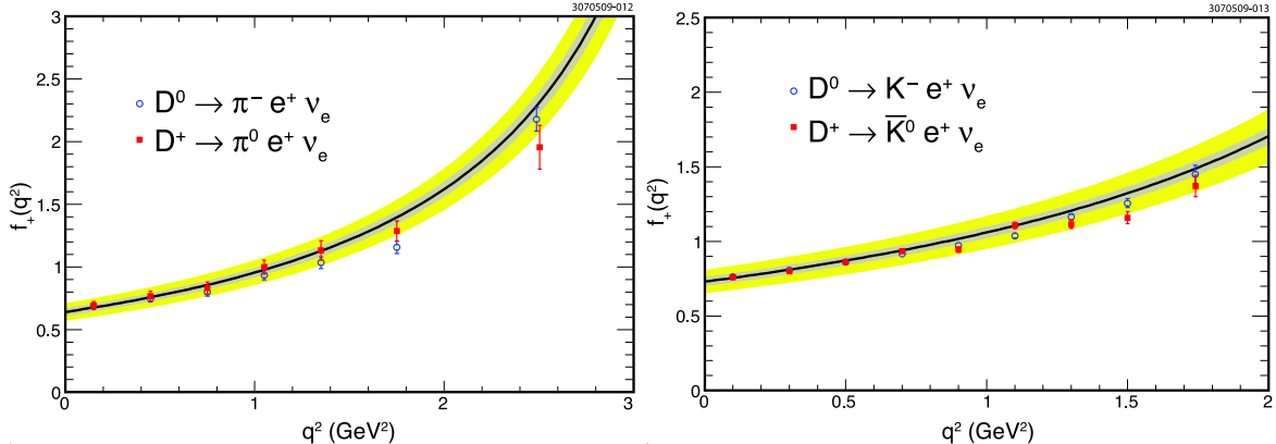
FIG. 8: f_+(q^2) comparison between isospin conjugate modes and with LQCD calculations [21]. The solid lines represent LQCD fits to the modified pole model [15]. The inner bands show LQCD statistical uncertainties, and the outer bands the sum in quadrature of LQCD statistical and systematic uncertainties.
