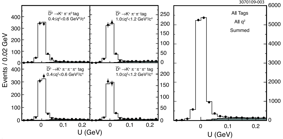
FIG. 3: U distributions in data (points) for D^0 \rightarrow K^- e^+ \nu_e , with fit results (histograms) showing signal (clear) and background components: D\bar{D} (gray) and non- D\bar{D} (black).
