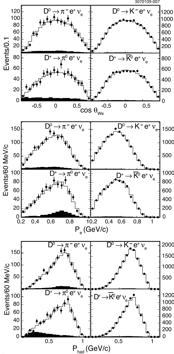
FIG. 7: Distributions of \cos \theta_{W_e} (upper), the cosine of the angle between the virtual W and the positron, positron momentum (middle) and hadron momentum (lower) in events satisfying -60 \text{ MeV} < U < 60 \text{ MeV} . Signal and background shapes are taken from MC simulations and scaled using the parameters of the signal yield fits.
