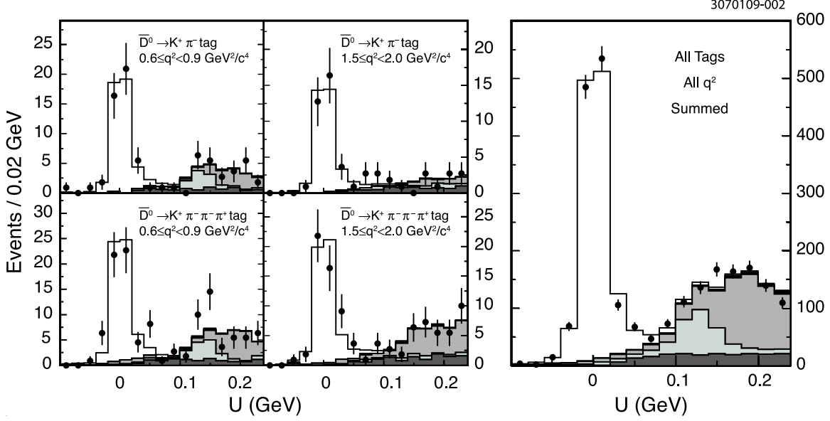
FIG. 2: U distributions in data (points) for D^0 \rightarrow \pi^- e^+ \nu_e , with fit results (histograms) showing signal (clear) and background components: D^0 \rightarrow \rho^- e^+ \nu_e (darkest gray), D^0 \rightarrow K^- e^+ \nu_e (lightest gray), other D\bar{D} (medium gray), and non- D\bar{D} (black).
