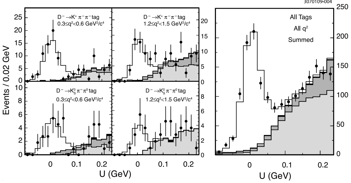
FIG. 4: U distributions in data (points) for D^+ \rightarrow \pi^0 e^+ \nu_e , with fit results (histograms) showing signal (clear) and background components: D^+ \rightarrow \bar{K}^0 e^+ \nu_e (light gray), other D\bar{D} (dark gray), and non- D\bar{D} (black).
