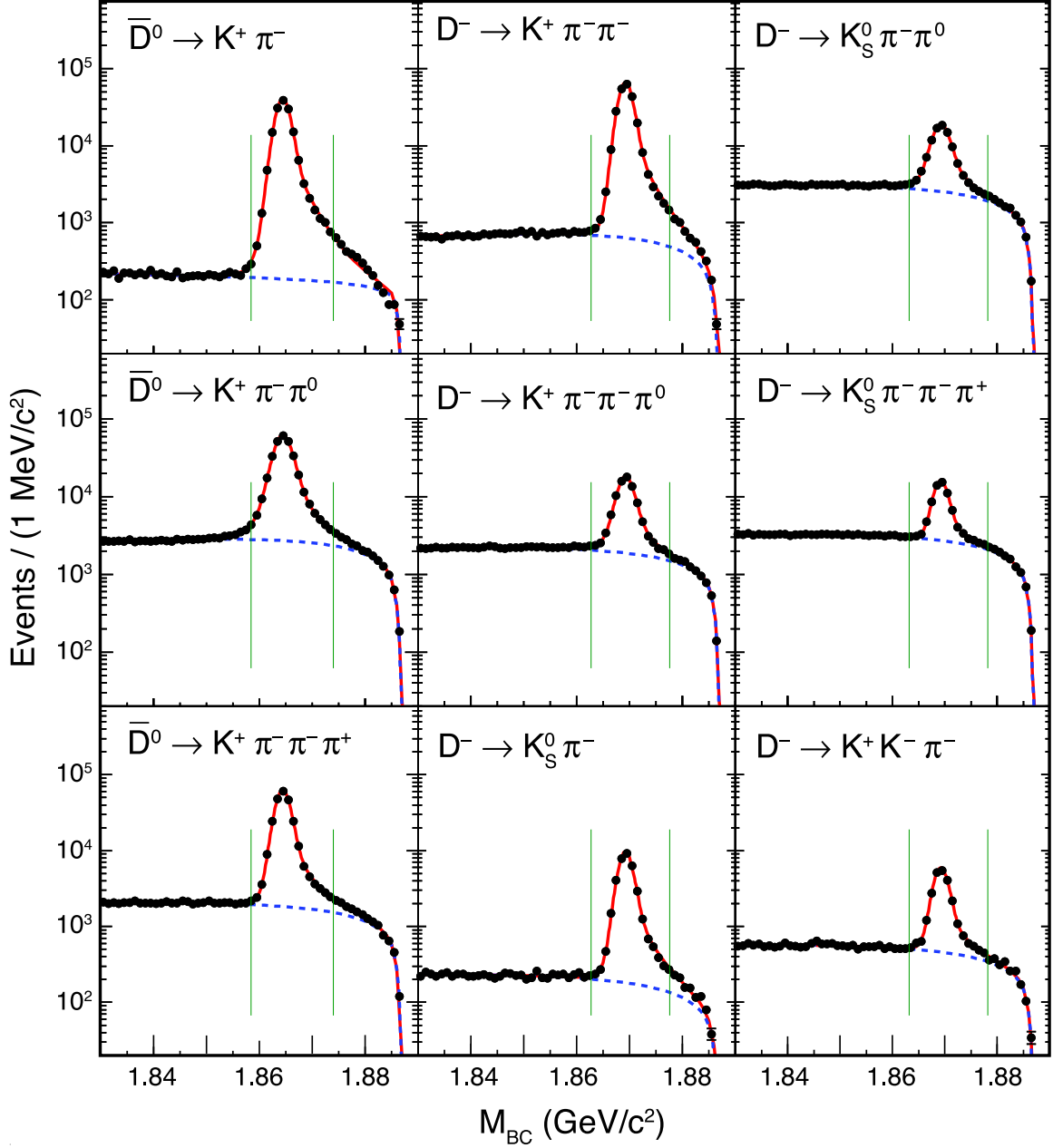
FIG. 1: M_{BC} distributions in data (points), with fits (solid lines) and background contributions to fits (dotted lines). The vertical lines show the limits of the M_{BC} signal regions.
