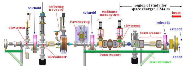
Figure 1: DC gun diagnostics beamline.
