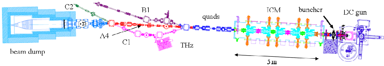
Figure 2: The layout of Cornell prototype ERL injector. Beam direction is to the left.
