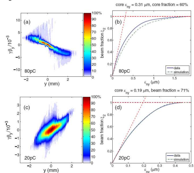
Figure 4: Measured (a), (c) transverse phase space after the gun and the corresponding emittance versus beam fraction curve (b), (d).
