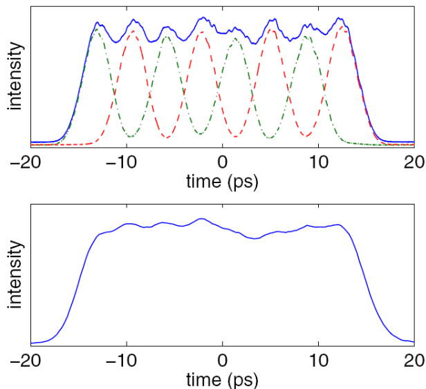
Figure 4: Laser pulse (top) and electron bunch (bottom) temporal profile measurement after three shaping crystals. Laser cross correlation shows the intensity of the two orthogonal polarizations (dashed and dot-dashed) and their sum (solid line).
