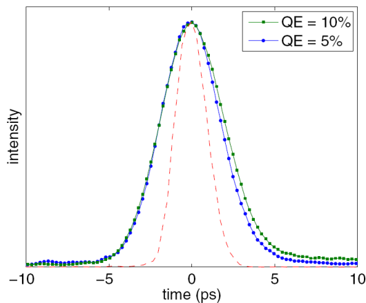
Figure 3: Temporal response obtained from GaAs excited by 1 ps rms 520 nm laser pulses. The dashed line shows the resolution of the measurement.
