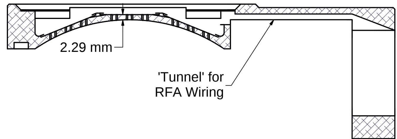
SECTION B-B SCALE 1 : 1
