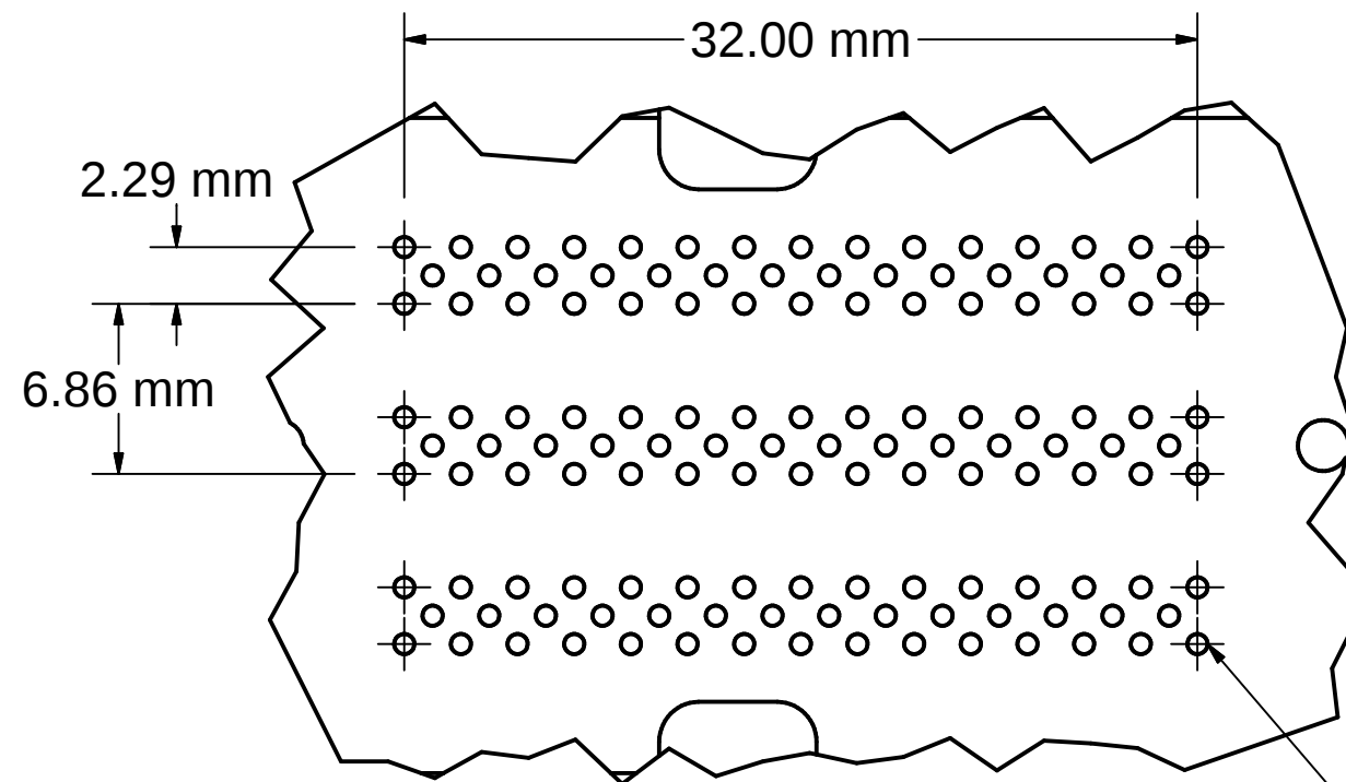
RFA HOLE PATTERN (Rotated)
