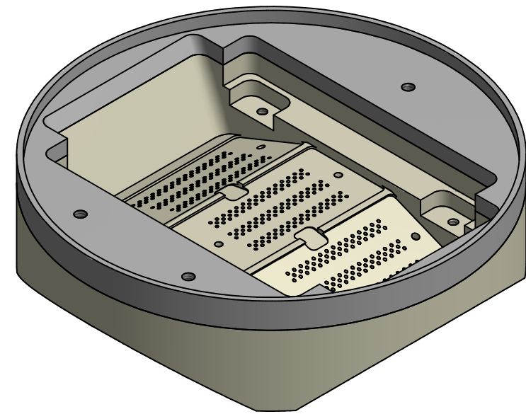
RFA Housing
