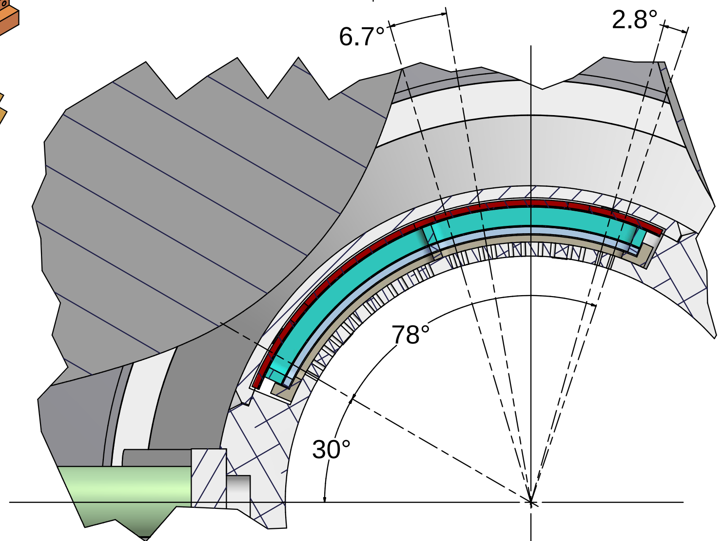
(DETAIL B) RFA Angular Dimensions
