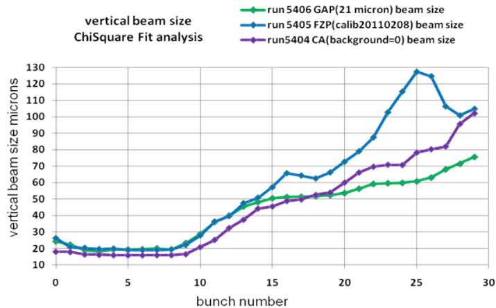
vertical beam size ChiSquare Fit analysis
