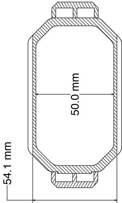
SECTION C-C SCALE 2
