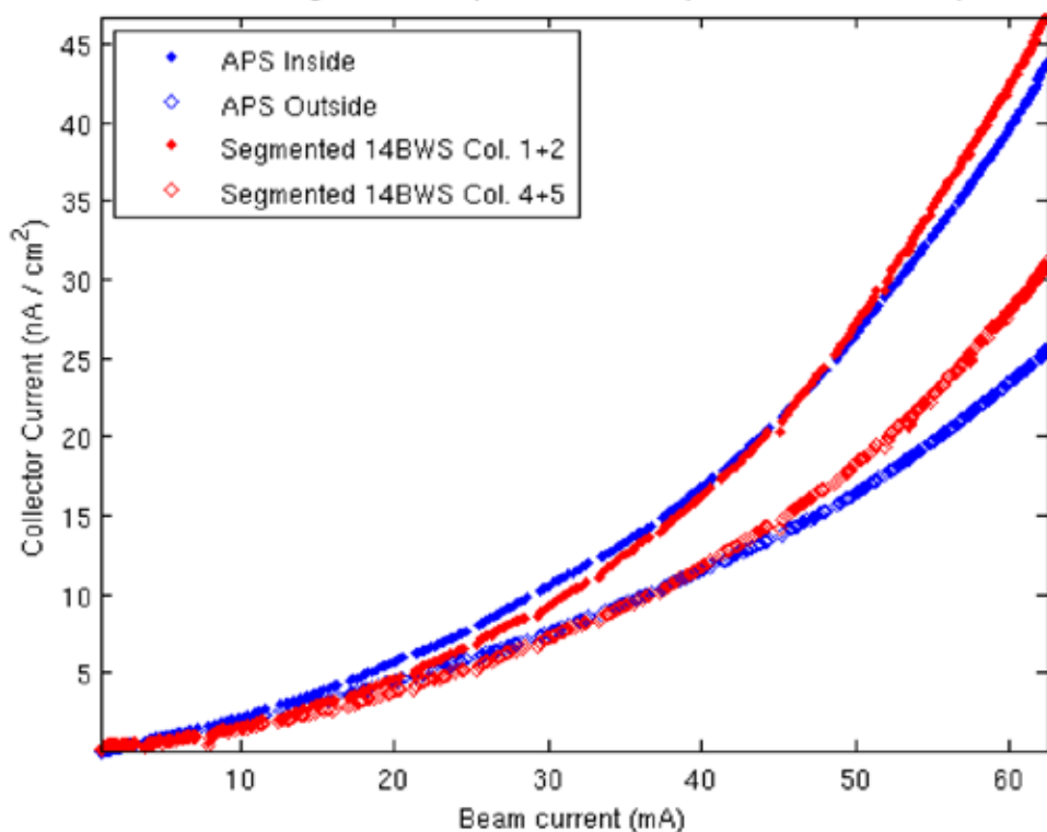
APS vs Segmented Comparison: run 675 (1x45x1.2mA e+)
