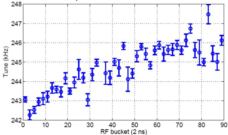
CESR-TA bunch-by-bunch tune, 45.6 mA, 45 bunches, mar1109/172917
