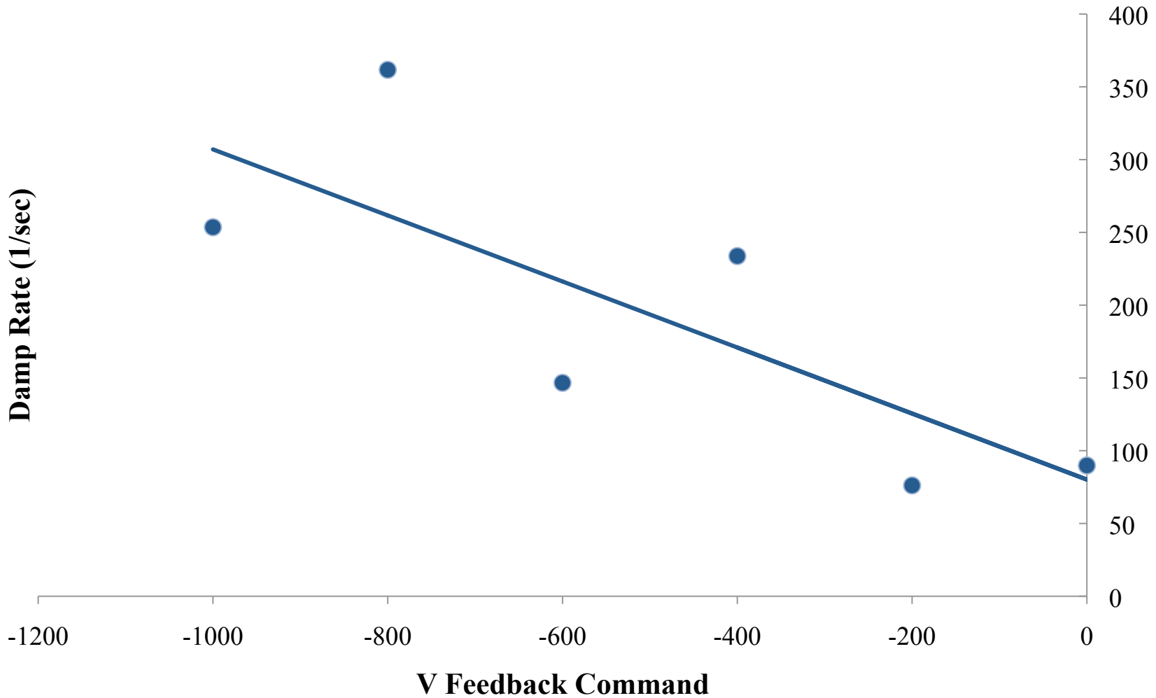
Damping Rate vs V Feedback Command (m=-1)
