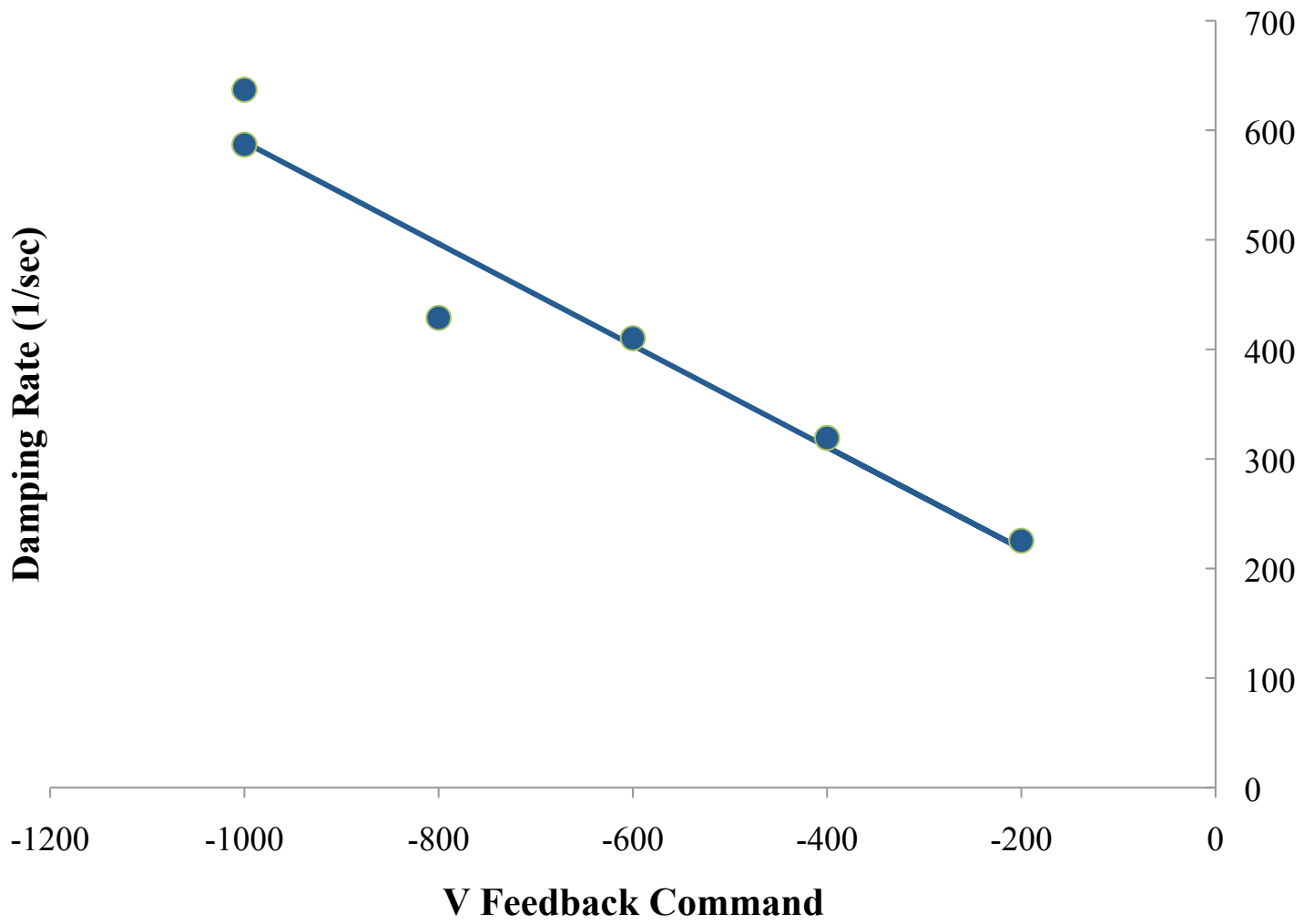
Damp Rate vs V Feedback Command (m=0)
