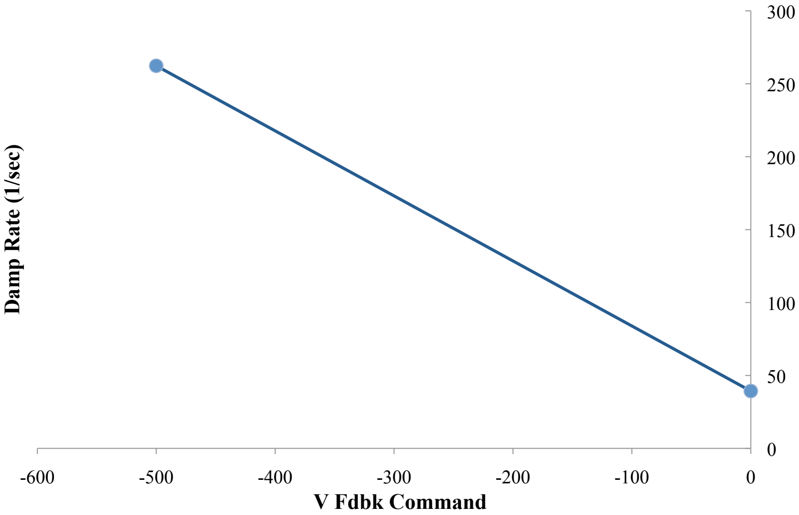
Damping Rate vs V Fdbk Command (m = +1)
