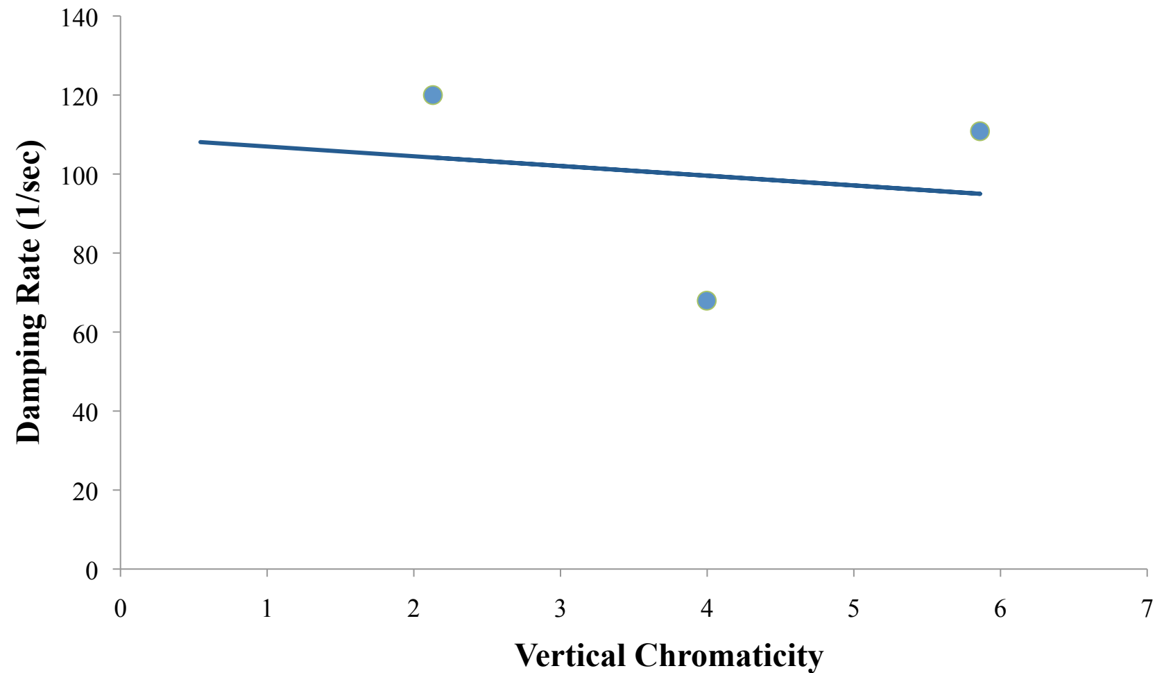
Damp Rate vs Vertical Chromaticity ( m = 0 )
