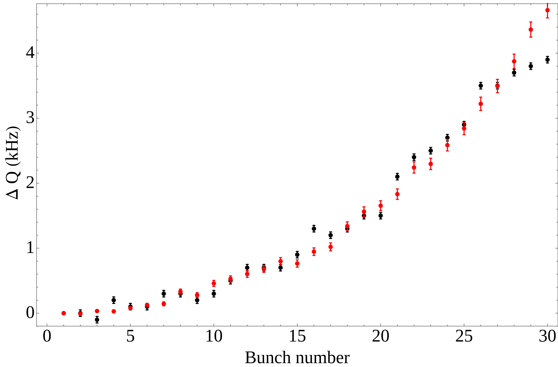
Horizontal Coherent tune shift vs. bunch number
