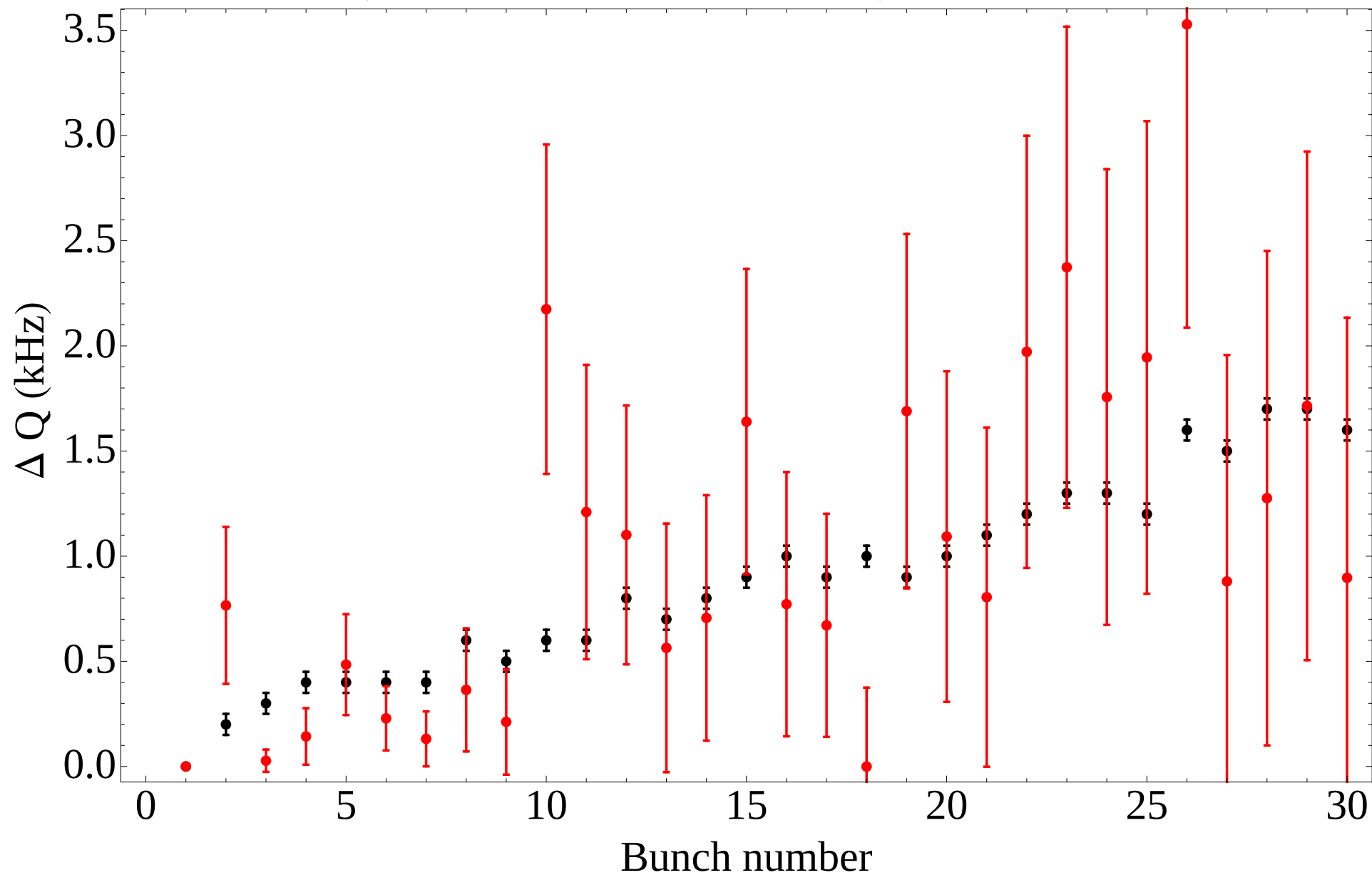
Vertical Coherent tune shift vs. bunch number
