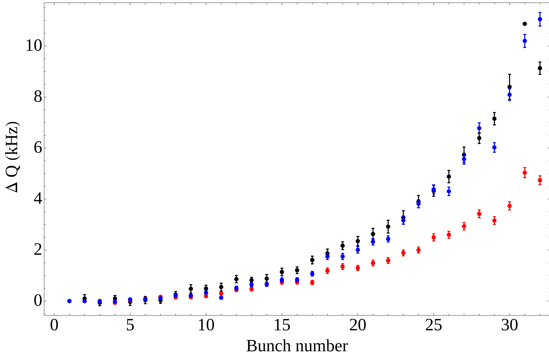
Horizontal Coherent tune shift vs. bunch number
