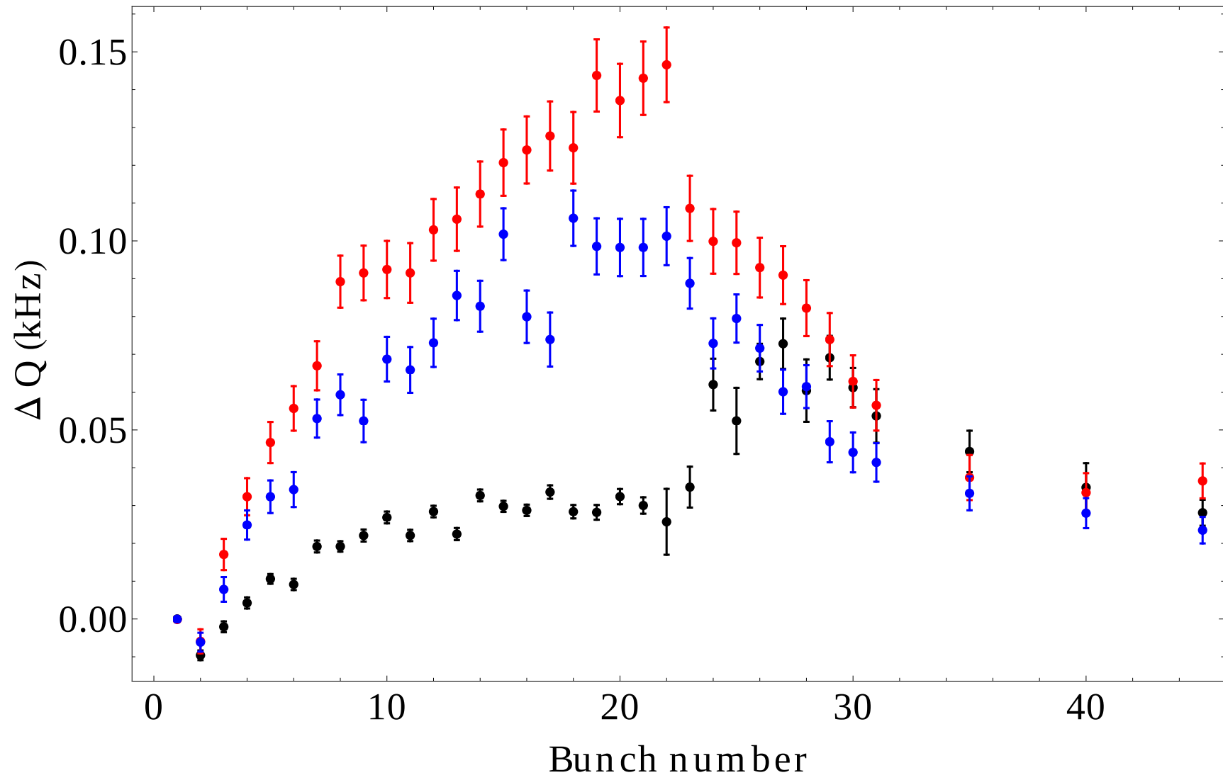
Horizontal Coherent tune shift vs. bunch number
