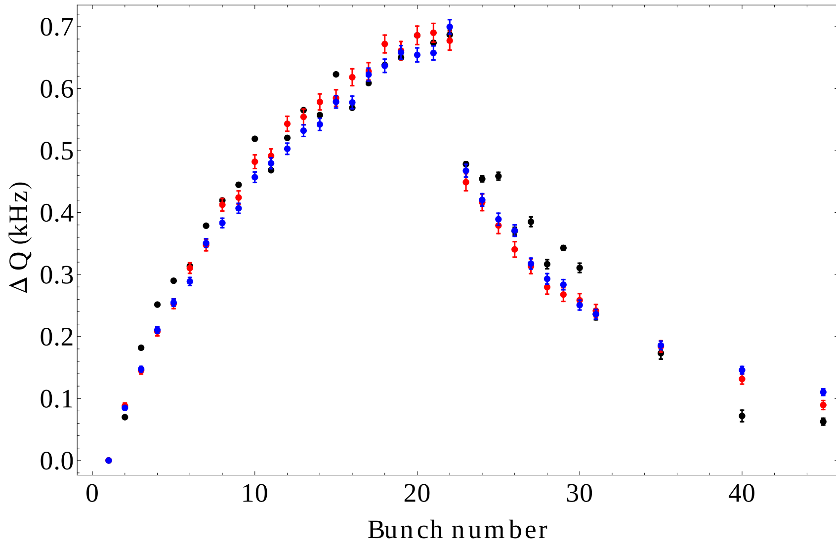
Vertical Coherent tune shift vs. bunch number
