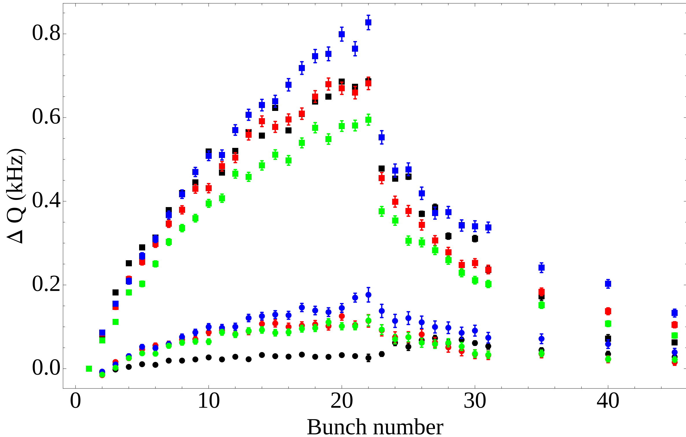
Coherent tune shift vs. bunch number
