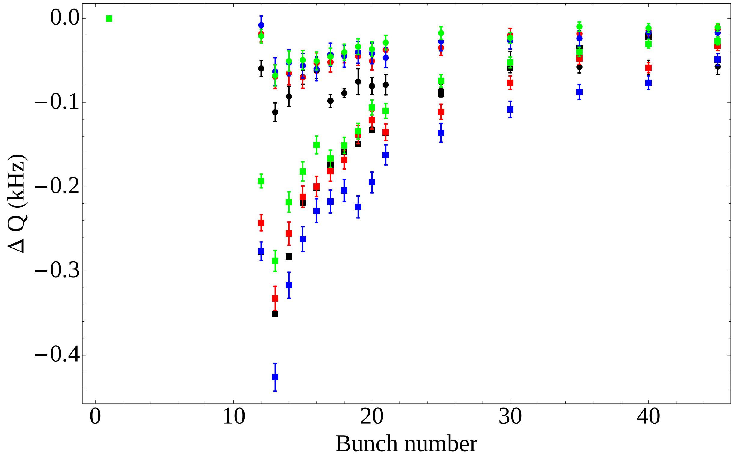
Coherent tune shift vs. bunch number
