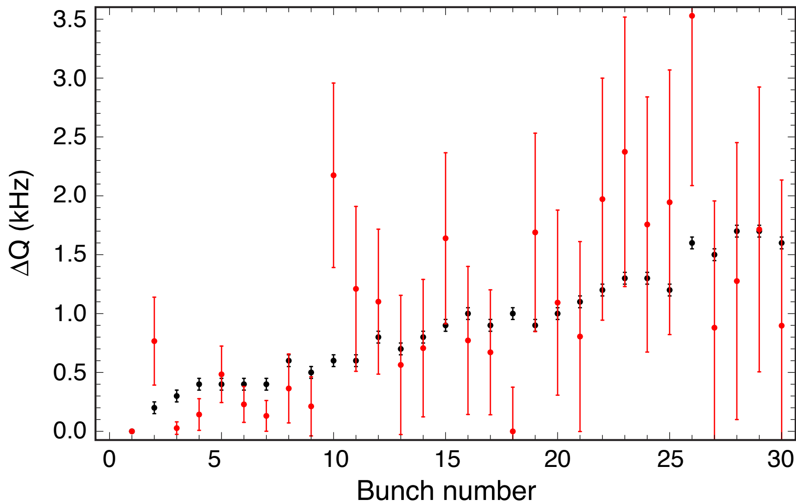
Vertical Coherent tune shift vs. bunch number
