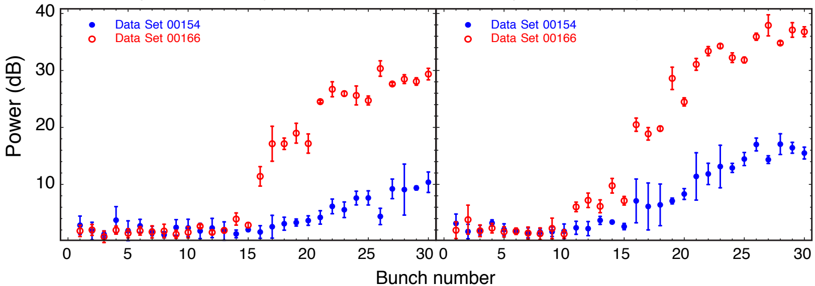
Relative power vertical synchrobetatron +1 line Relative power vertical synchrobetatron -1 line
