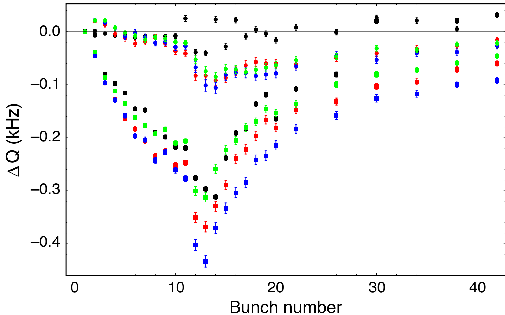
Coherent tune shift vs. bunch number
