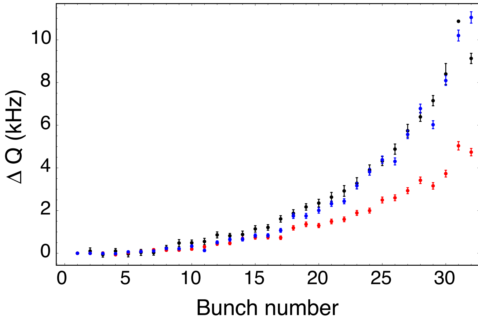
Horizontal Coherent tune shift vs. bunch number
