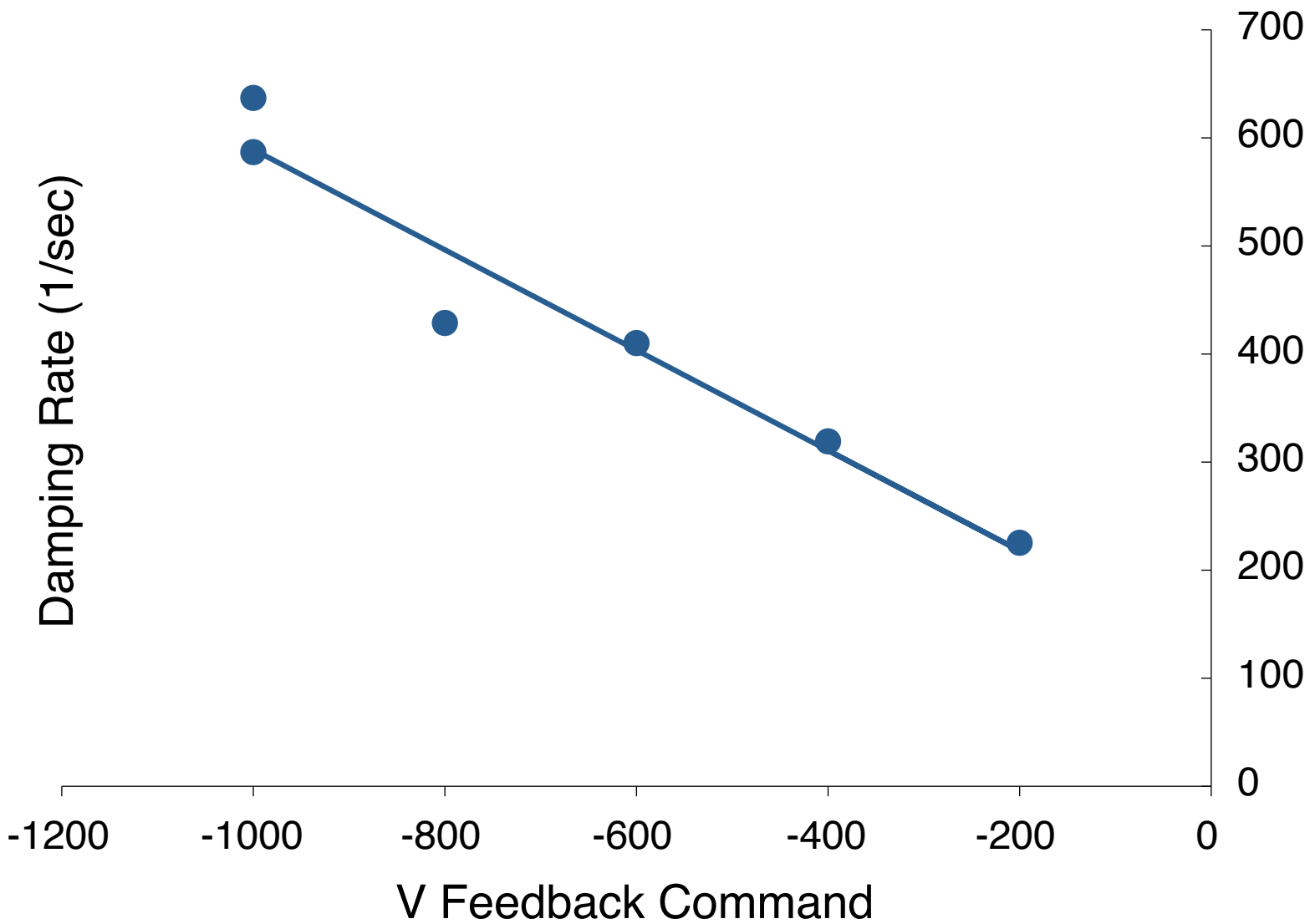
Damp Rate vs V Feedback Command (m=0)
