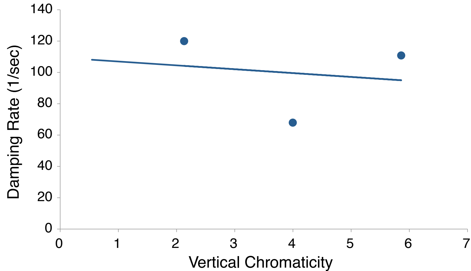
Damp Rate vs Vertical Chromaticity ( m = 0 )
