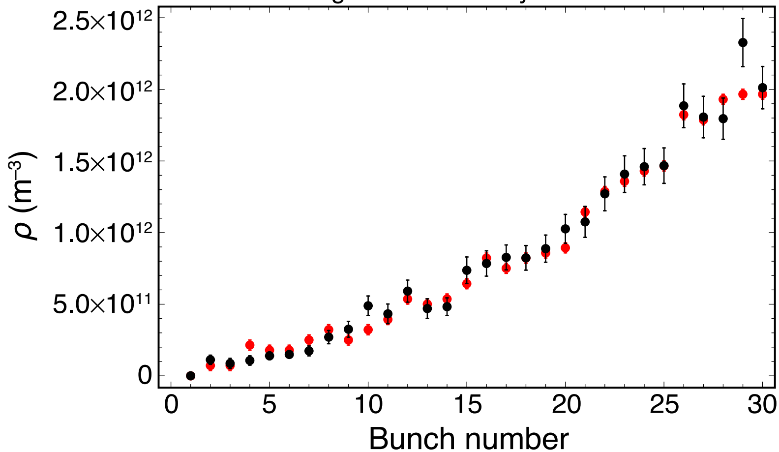
Beam averaged cloud density vs. bunch number
