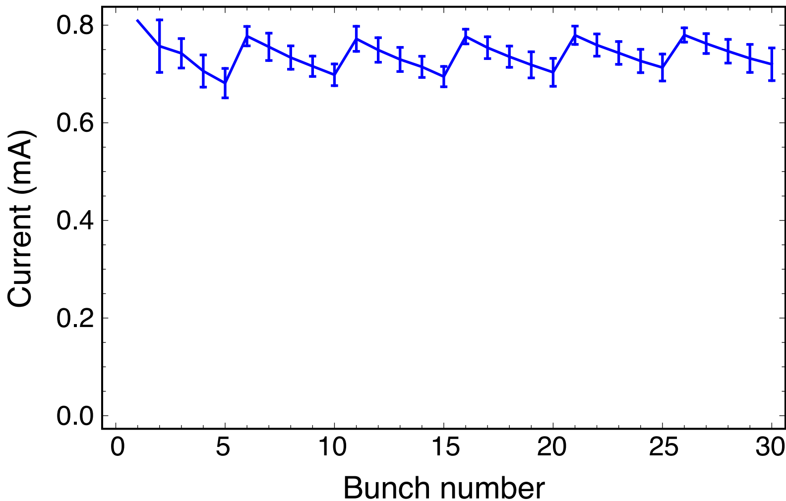
Bunch currents: Data set 00166
