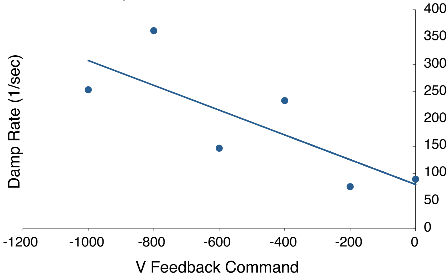
Damping Rate vs V Feedback Command (m=-1)
