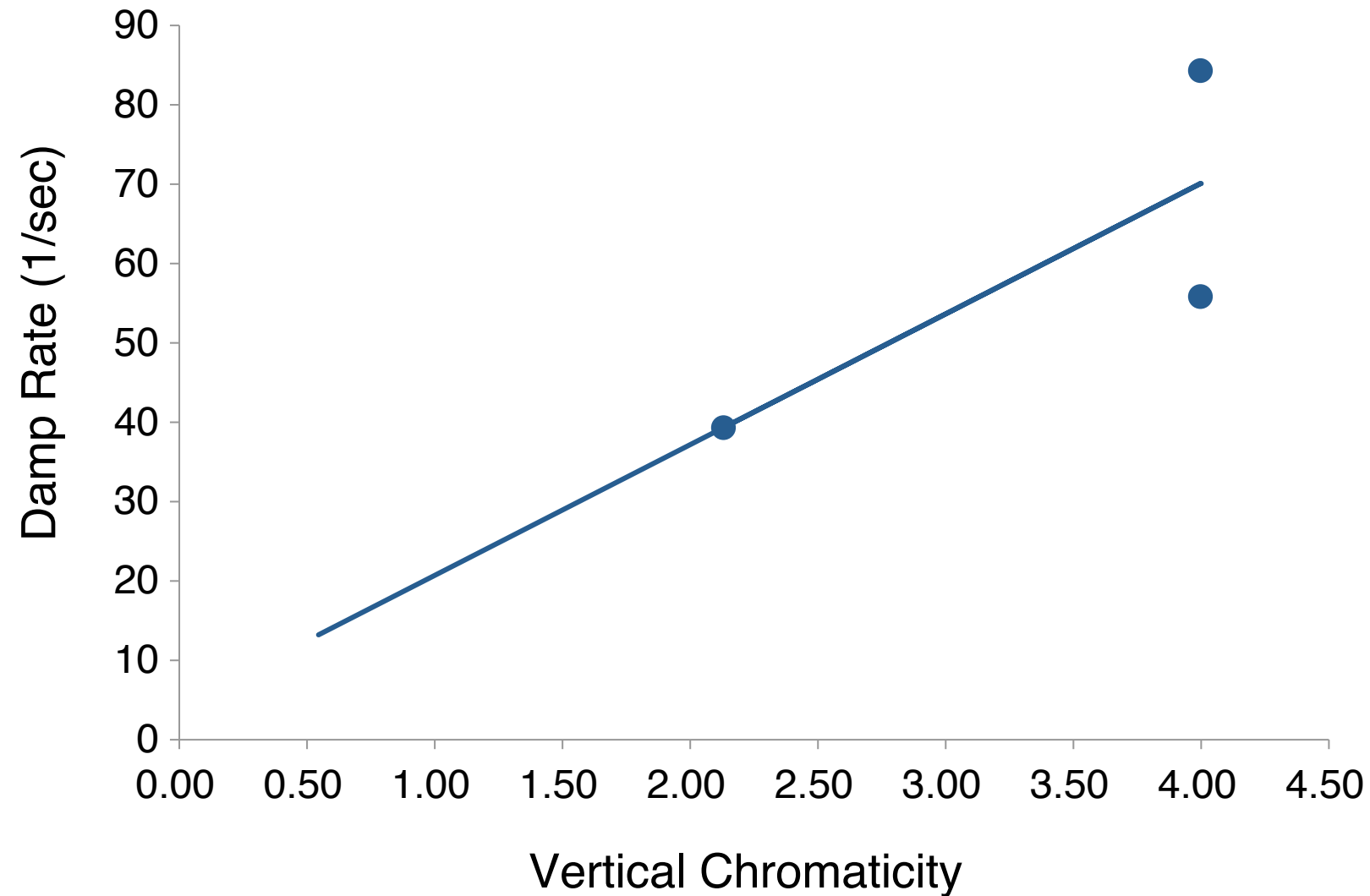
Damping Rate vs Vertical Chromaticity ( m = +1 )
