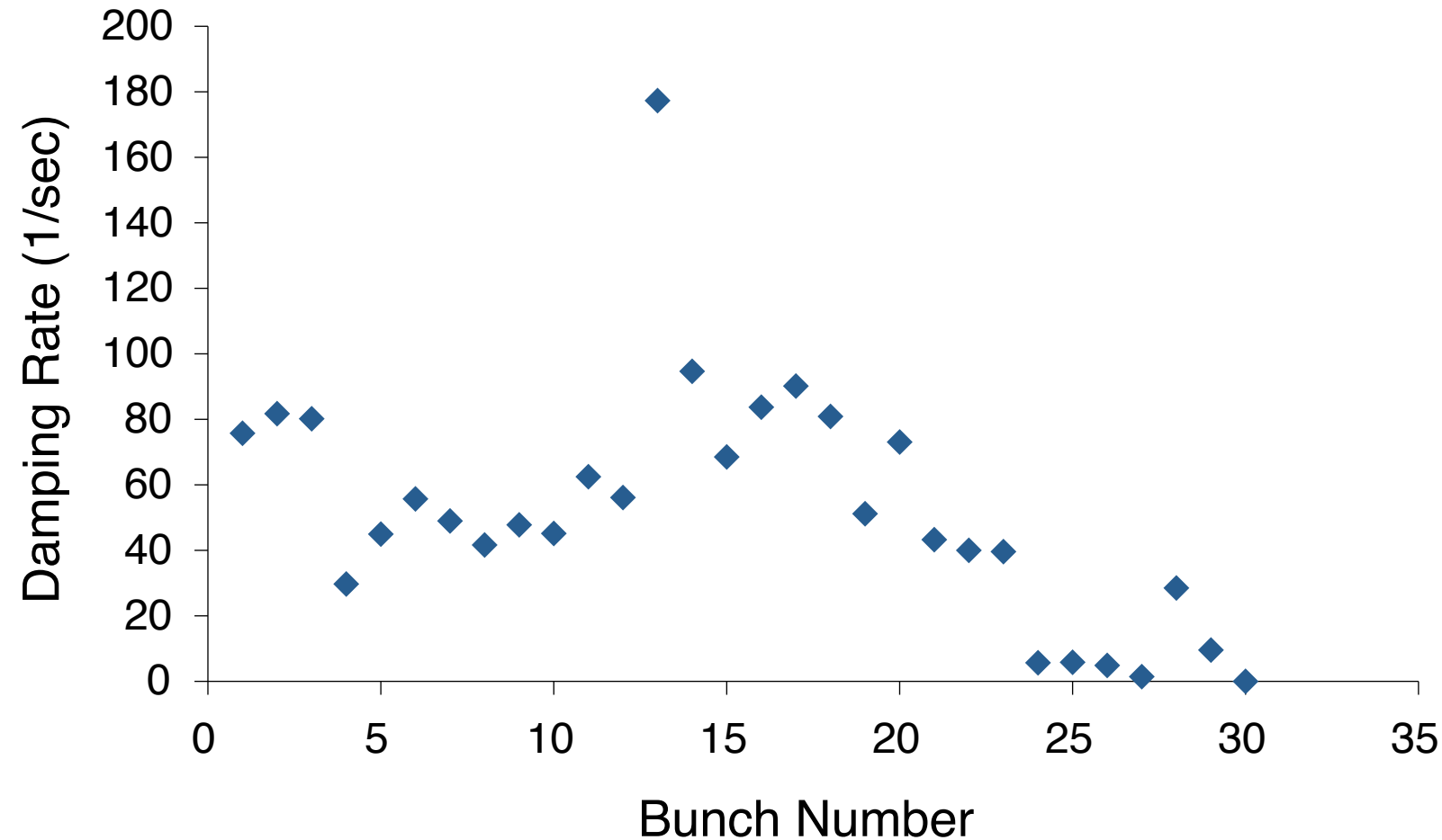
Damping Rate vs. Bunch Number
