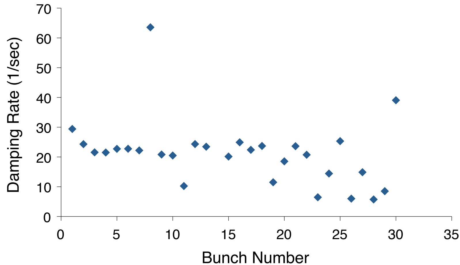
Damping Rate vs. Bunch Number
