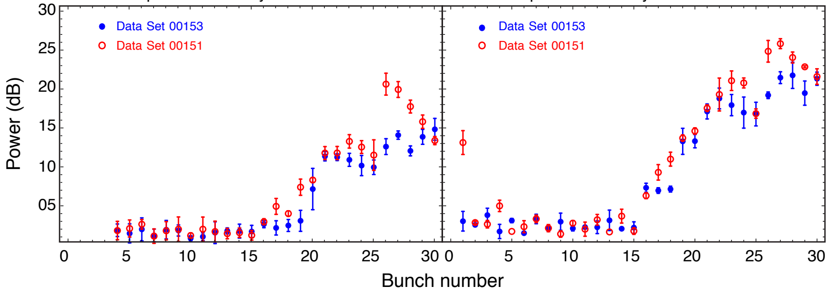
Relative power vertical synchrotron +1 line
