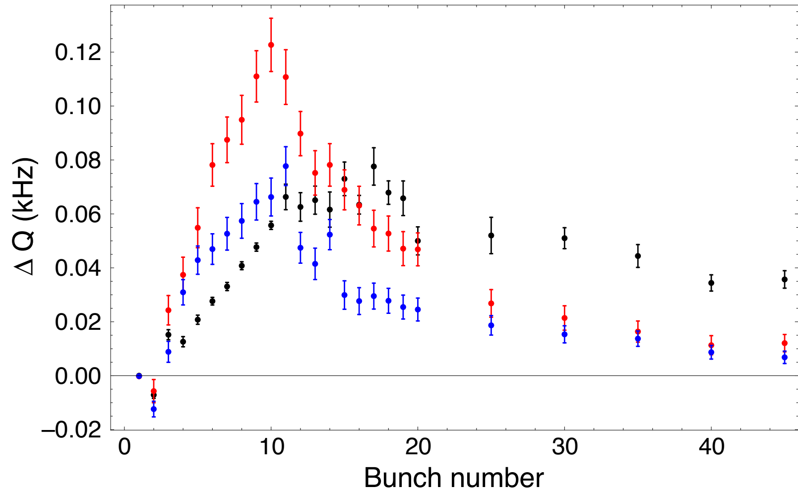
Horizontal Coherent tune shift vs. bunch number
