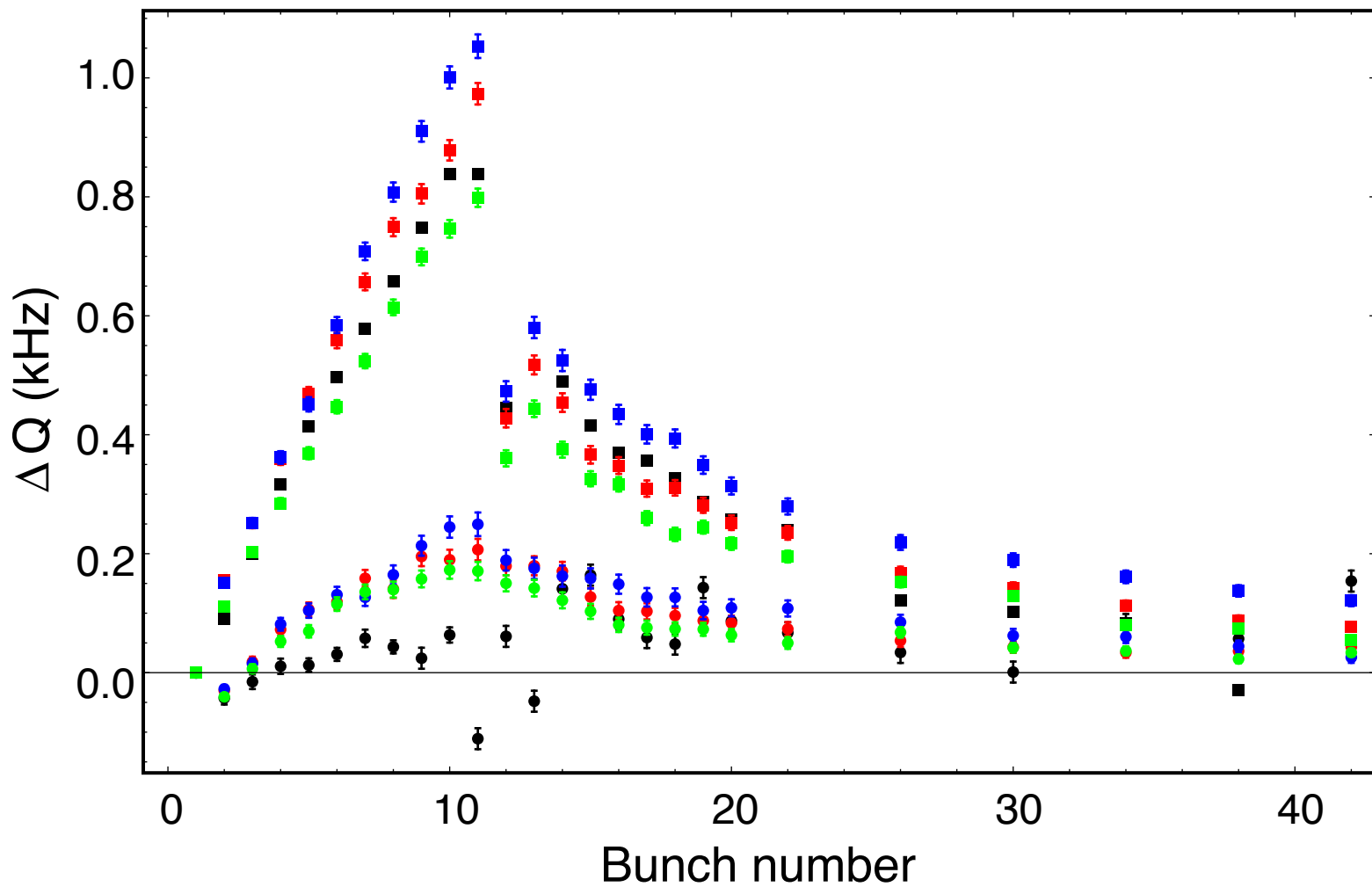
Coherent tune shift vs. bunch number
