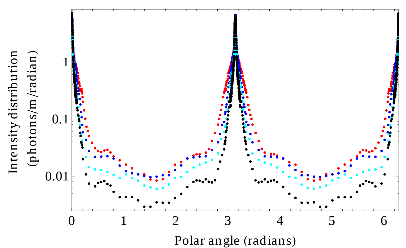
WIGGLER
