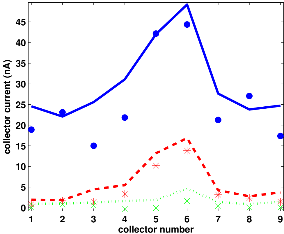
9 Bunches, 3.8mA, e+, 280ns, 2.1GeV
