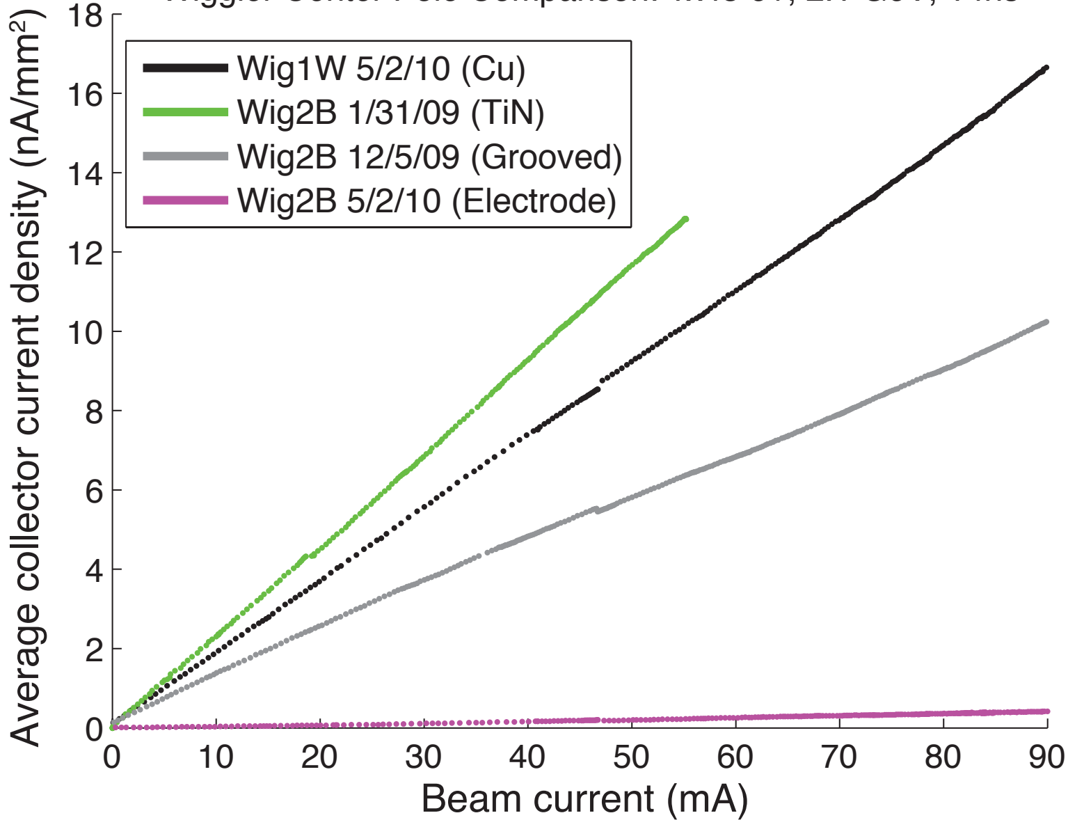
Wiggler Center Pole Comparison: 1x45 e+, 2.1 GeV, 14ns
