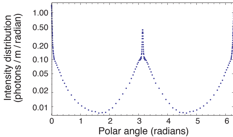
WIGGLER
