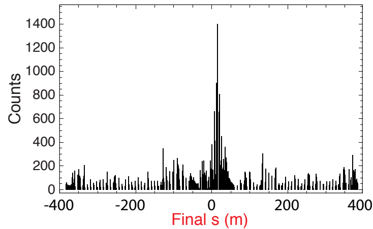
WIGGLER
