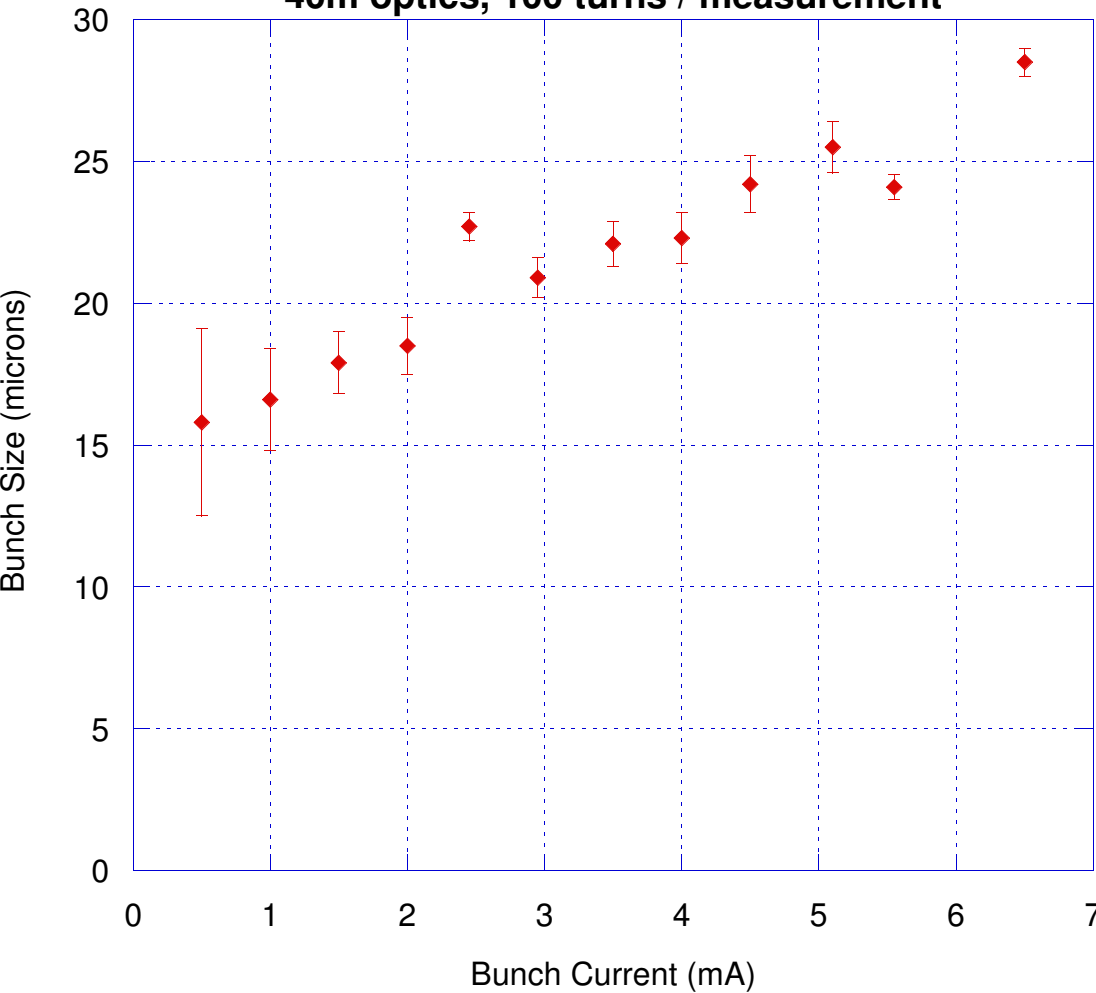
Bunch Size vs. Current 40m optics, 100 turns / measurement
