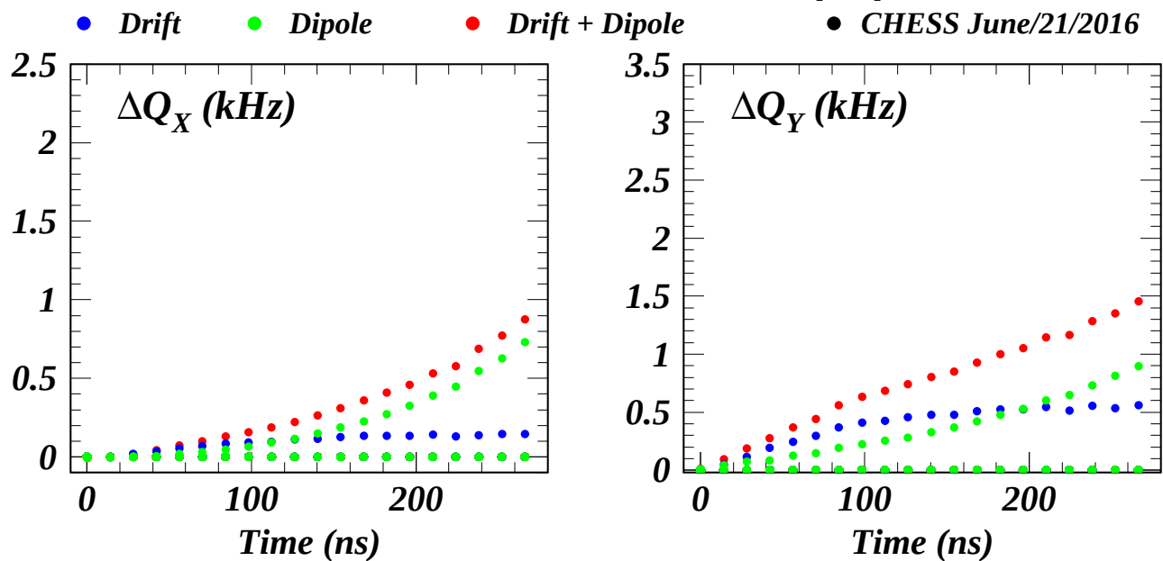
CH20160621_1mA_14ns: Coherent Tune Shifts for Jobs 42386/42387
