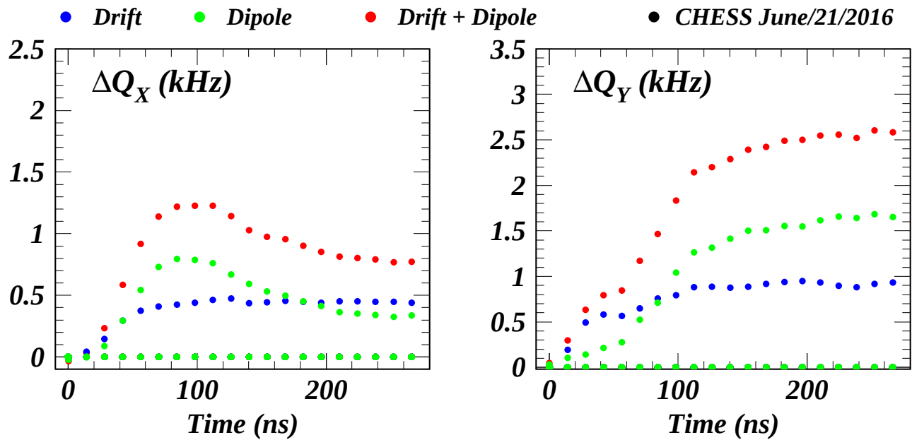
CH20160621_4mA_14ns: Coherent Tune Shifts for Jobs 42390/42391
