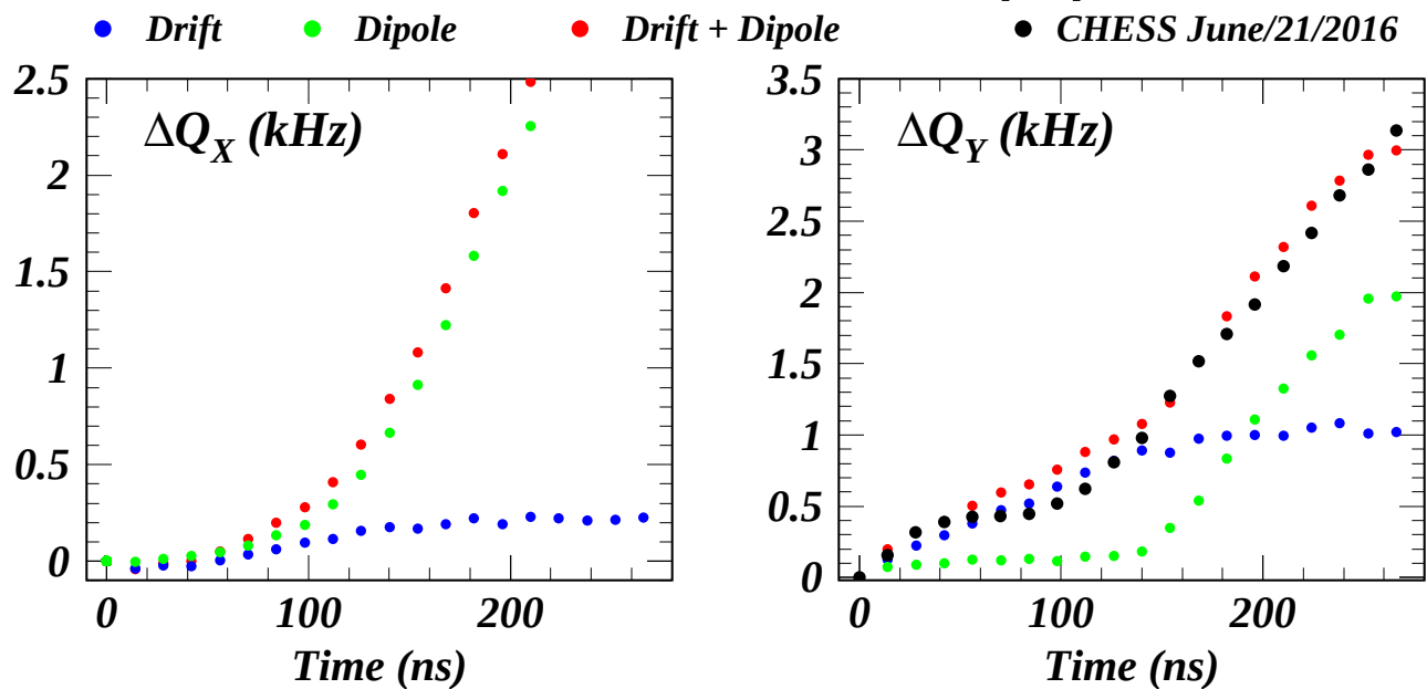
CH20160621_2mA_14ns: Coherent Tune Shifts for Jobs 52531/52532
