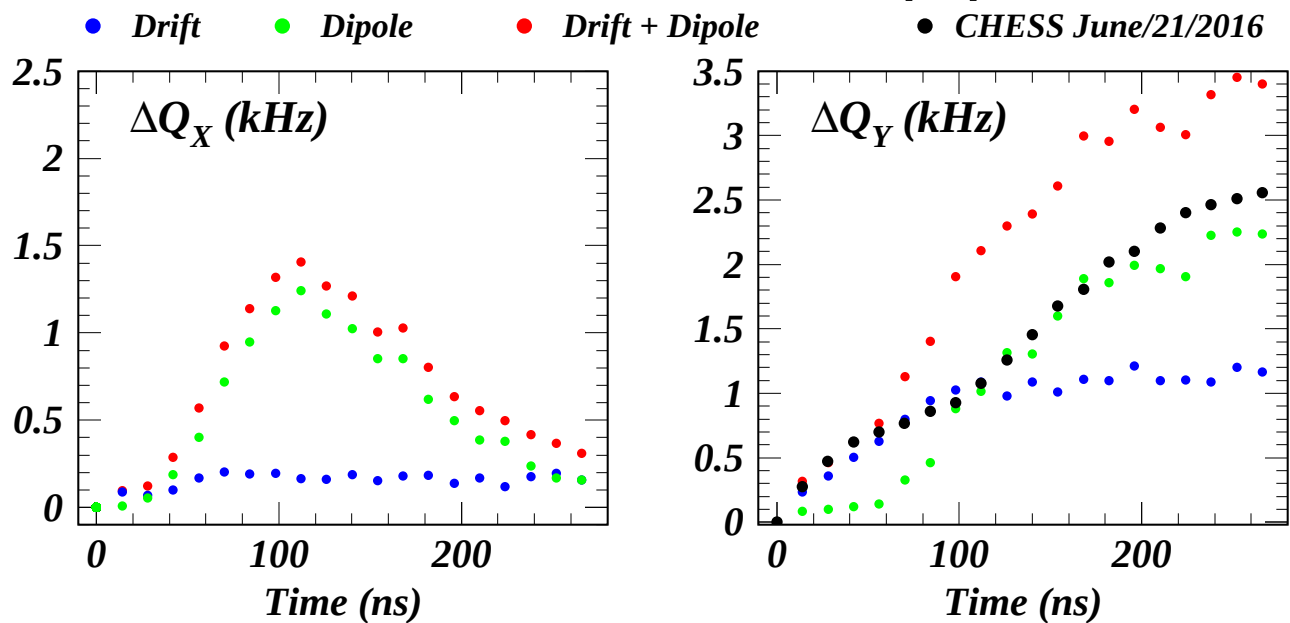
CH20160621_4mA_14ns: Coherent Tune Shifts for Jobs 52543/52544
